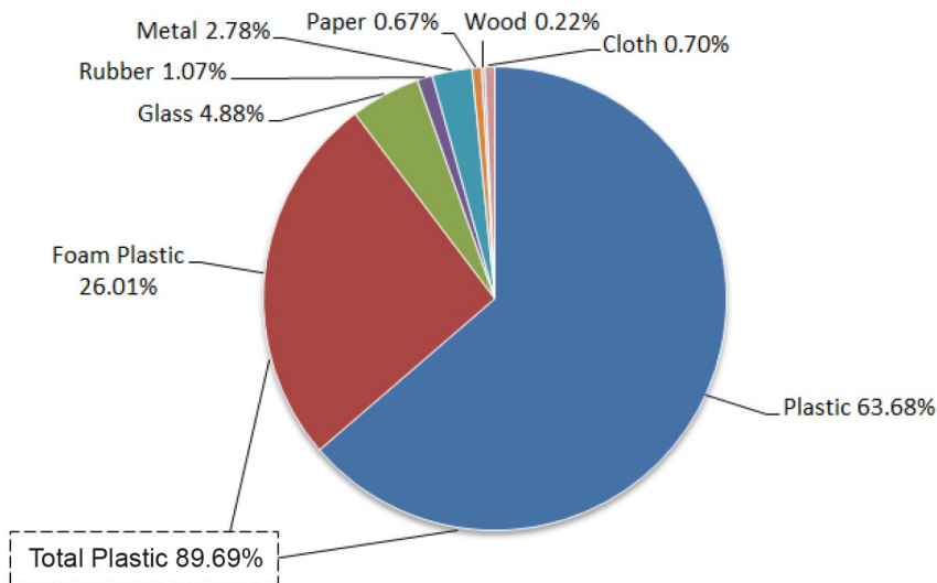
Figure 2. Breakdown of total debris collected at four locations along the Delaware River from 2016-2019 by material. Nearly 90% of collected debris is plastic, and foam plastic comprises over a quarter of total debris.
