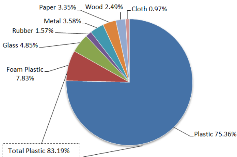
Figure 3. Breakdown of total debris collected at 62 locations, primarily along the Jersey Shore, during the 2019 Beach Sweeps by material. While the vast majority of the debris is plastic, foam plastic is less prevalent along the Jersey Shore as compared to the Delaware River.
